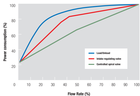
Performance Comparison of Air Compressor
